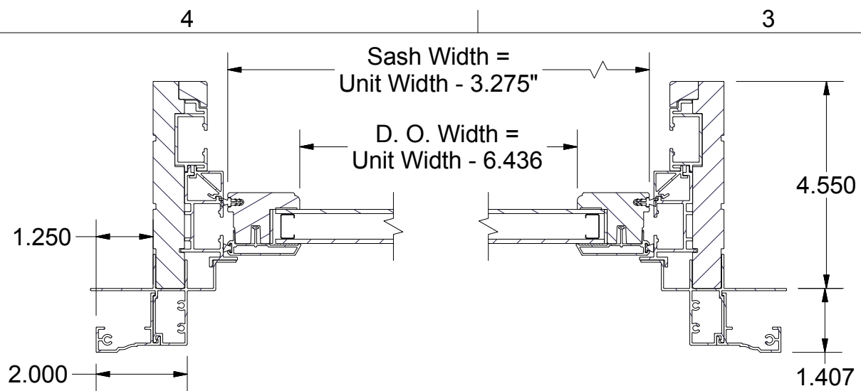
SECTION A-A SCALE 1 / 3
